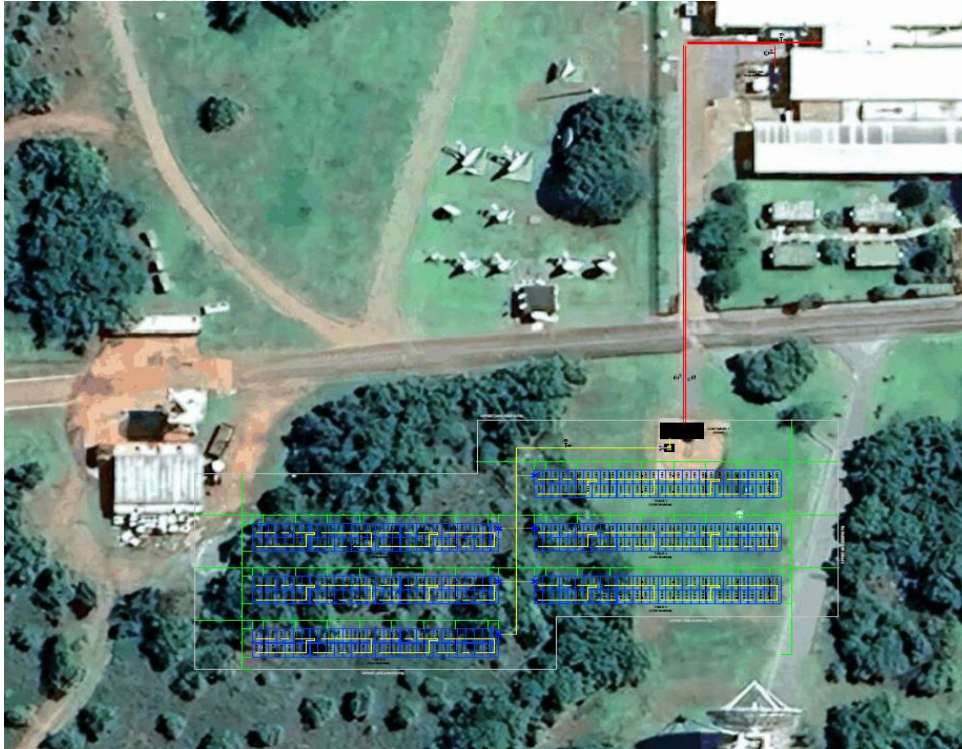
Figure 2: Hybrid 200kWp PV system
