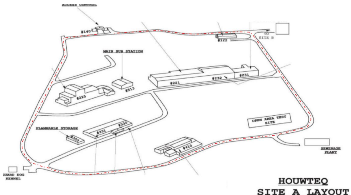
Figure 2: Houwteq AIT facility main campus layout of existing electric fence
