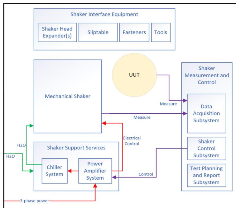
Figure 1: Mechanical vibration equipment scope and architecture
