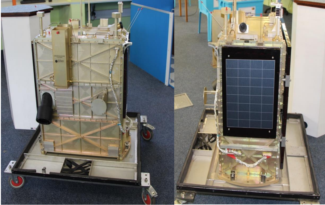
Exhibit 1: SumbandilaSAT Satellite Model
